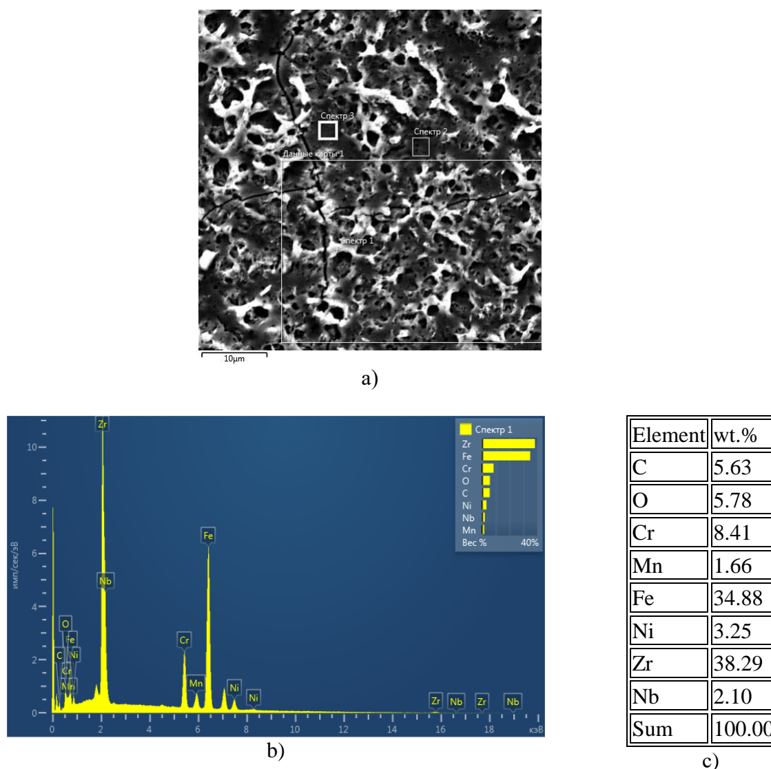
Fig. 1. SEM-image (a), EDAX spectrum (b) and element concentration (c) of the multi-element coating before electron beam treatment
