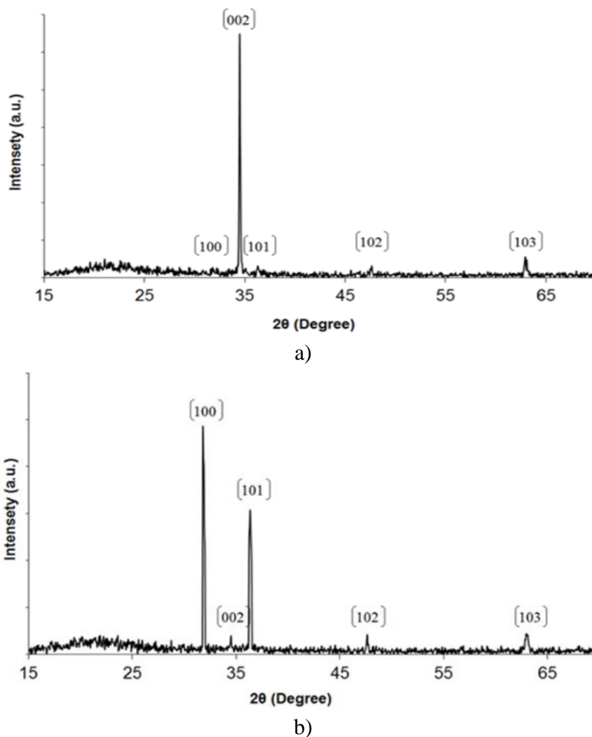
Fig.4. XRD analysis of ZnO NRs (a) and ZnO NSs (b)
