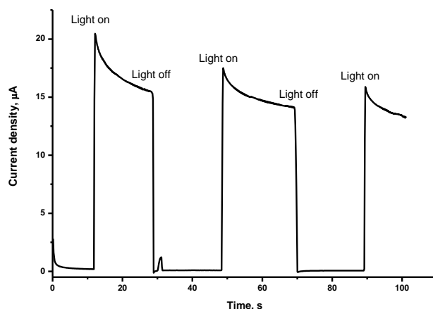
Fig.6. Photocurrent of bare ZnO nanosheets. 100W UV Xenon lamp was exploited as light source.
