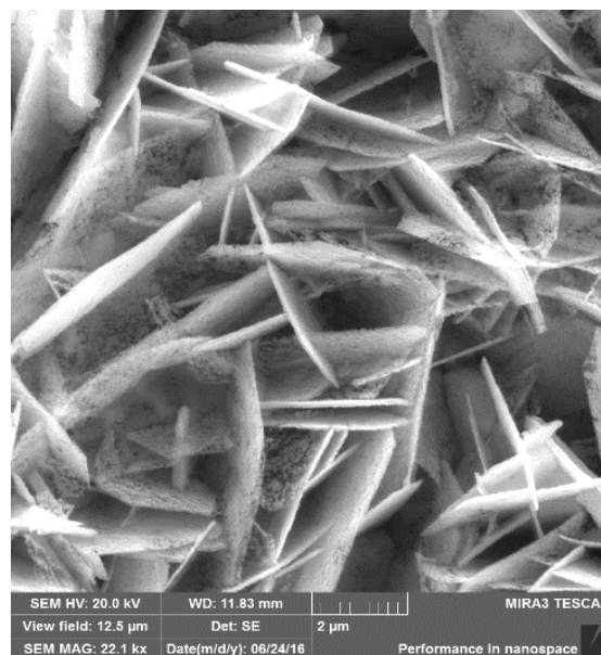
Fig.2. SEM image of ZnO NSs electrochemically deposited onto ITO glass
