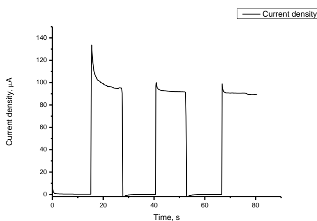
Fig.7. Photocurrent of ZnO/Fe 2 O 3 nanocomposites. 100W UV Xenon lamp was exploited as light source
