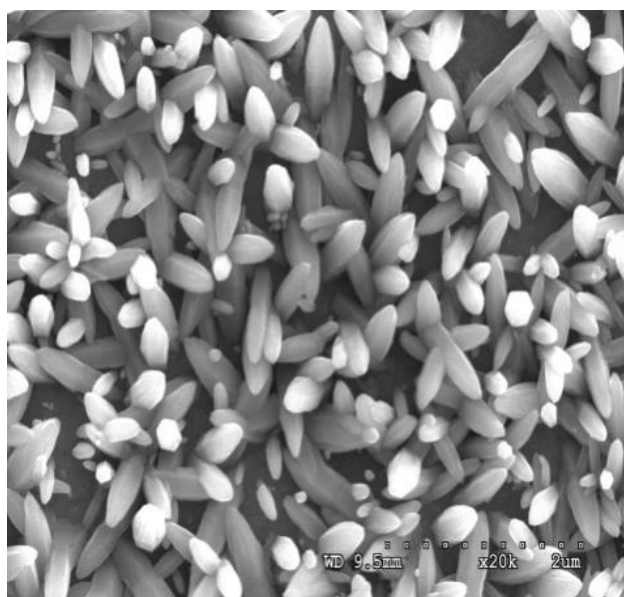
Fig.1. SEM image of ZnO nanorods arrays electrochemically deposited onto ITO glass
