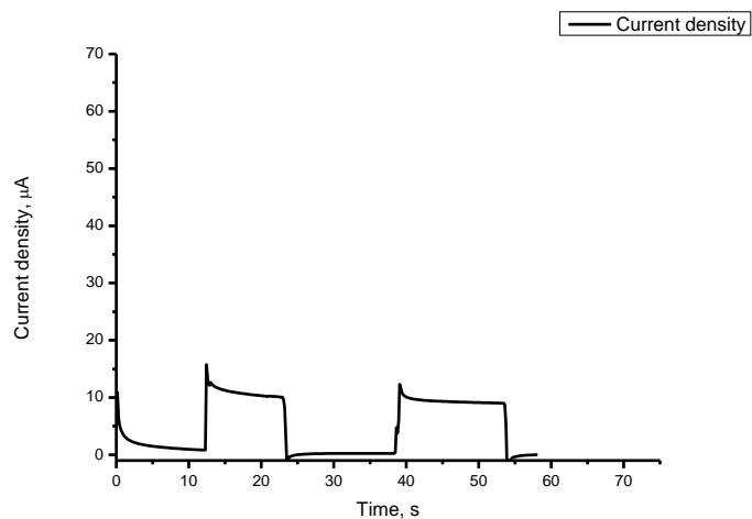
Fig.5. Photocurrent of bare ZnO nanorods. 100W UV Xenon lamp was exploited as light source
